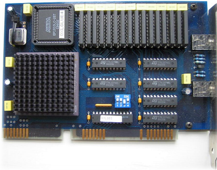
A QXL card
