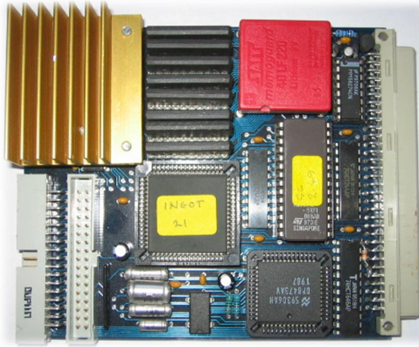
A Super Gold Card
