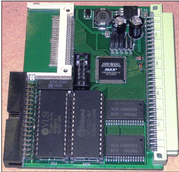
Prototype of Tetroid's new Trump Card with Qubide clone and Compact Flash
