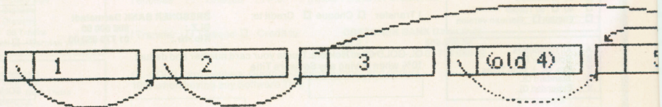
LINKED LIST SHOWING NEW ITEM 4.
